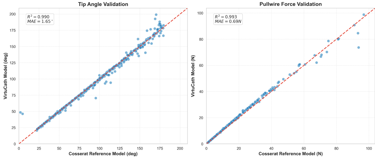
1-Segment Dataset Parity Plot
