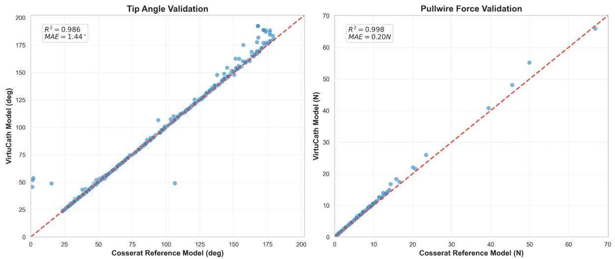
3-Segment Dataset Parity Plot
